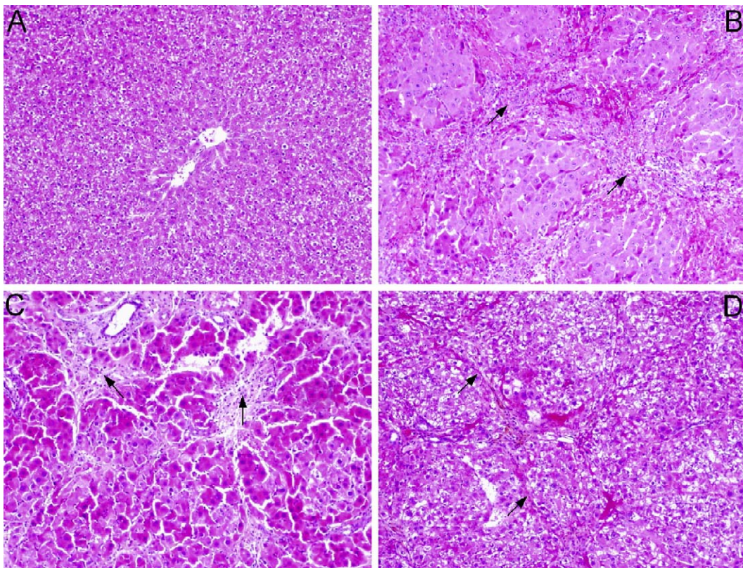
Fig. 2. Hematoxylin and eosin (H&E) staining of rat liver tissue during the pathogenesis of DMN-induced hepatic fibrosis. All days indicated are after the start of DMN administration ( \times 100 ). (A) Normal liver. (B) Day 7. Massive hepatic necrosis, multifocal collapse of the liver parenchyma (arrows), severe centrilobular congestion and dilatation of sinusoids with focal hemorrhage. (C) Day 14. Well developed fibrosis and early cirrhosis with multifocal hepatocyte necrosis and neutrophilic infiltration (arrows). (D) Day 21. Well developed cirrhosis with collagen fibers (arrows).
