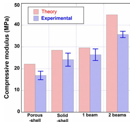
Fig. 9 Elastic modulus of theoretical and experimental results of PLLA scaffolds
